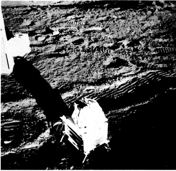
FIGURE 5-3. — Solar-wind spectrometer experiment deployed on the Moon.
