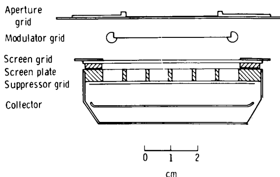
FIGURE 5-1. — Faraday-cup sensor.
